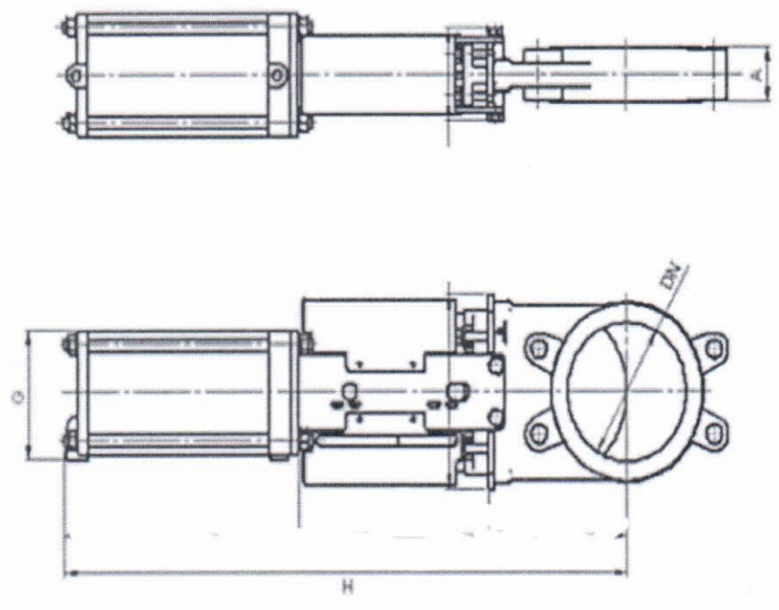
Valve Drawing
